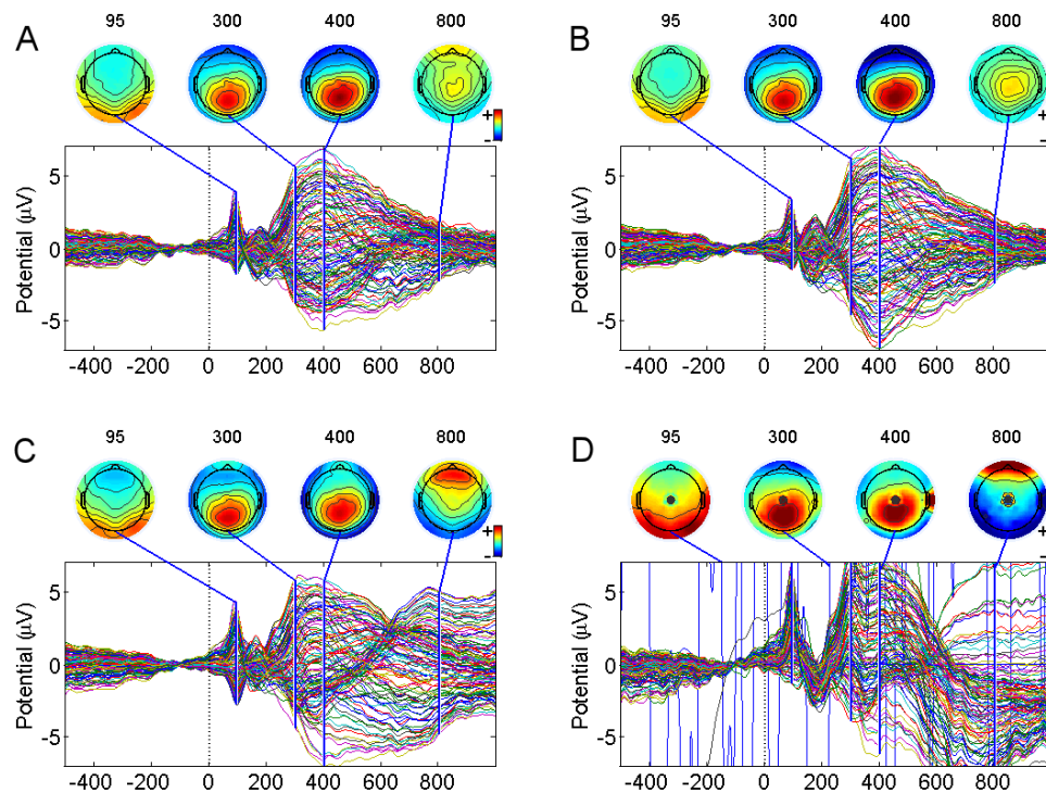
Figure 6. Butterfly plots of ERPs after various processing methods. A: supervised processing. B: FASTER processing. C: SCADS processing. D: Filter only. The late frontal
