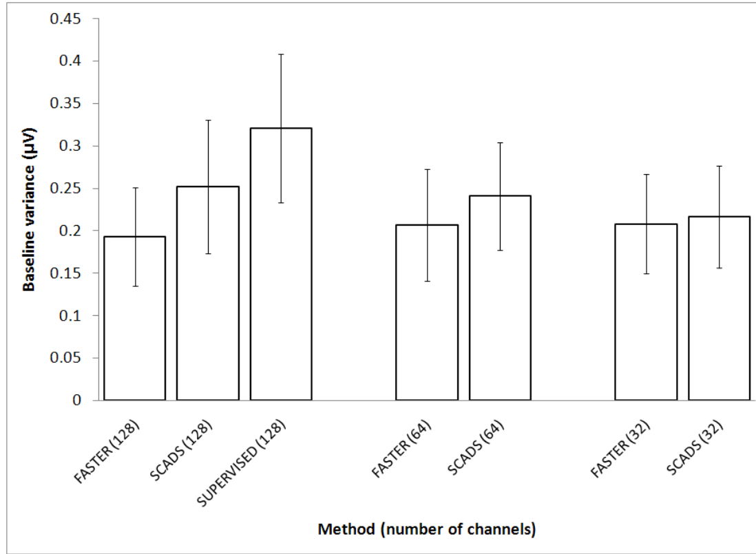
Figure 5. The baseline variance of different array sizes between FASTER, SCADS and supervised. Values shown are median and error bars display the interquartile range.
