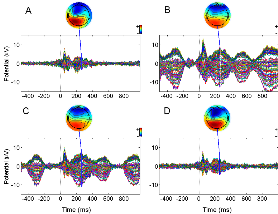
Figure 3. The ERPs calculated from simulated data with a different amount of artifacts present. A: the ERP from the dataset before artifact addition, B: the ERP after addition of all artefact types (see text for details), C: the ERP at 50% sensitivity, D: the ERP after complete removal of all artifacts (i.e., a 100% sensitivity).
