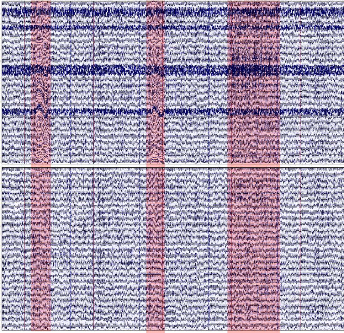
Figure 1. A section of a dataset with simulated artifacts added (top) and after removal with FASTER (bottom). Two EOG artifact and one EMG portion added to the data are highlighted. These have been removed in the bottom panel. A number of noise-contaminated channels are also present in the top panel, which have been corrected in the lower panel. This represents a 100% sensitivity (i.e. all artifacts removed) and 100% sensitivity (i.e. no uncontaminated channels or epochs removed) in the three epochs shown.
